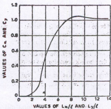
C-3 - Warping Stress Coefficient
